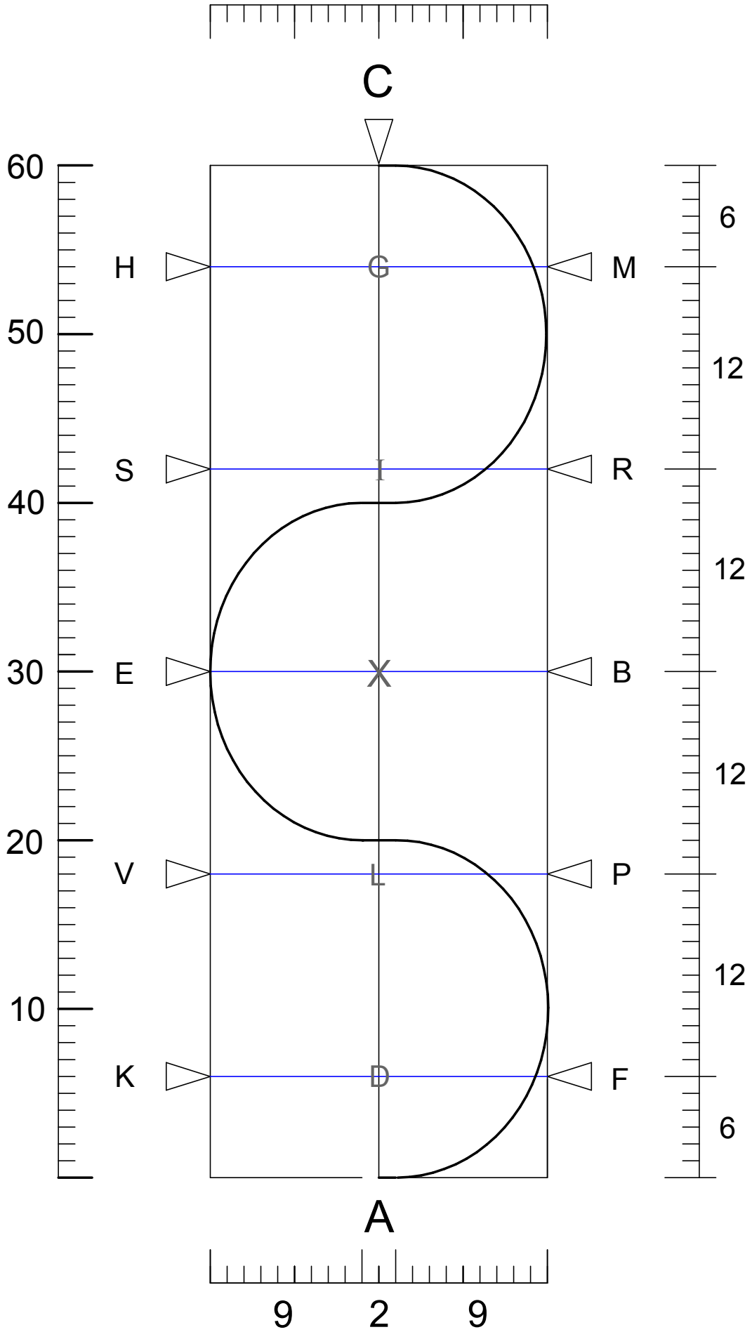
3 Equal loop Serpentine Centerline at A, 20 m, 40 m, & C. Sides at 10m, E, & 50m
